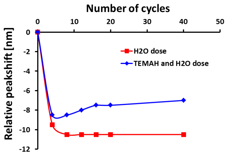
Fig. 3 Measured relative peak shift of the 1D PC with TEMAH and H 2 O and only H 2 O dose sequences
