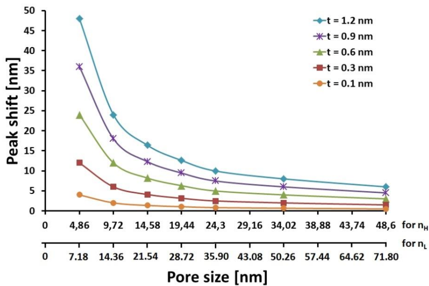
Fig. 2 Simulated peak shift as a function of the pore size for n_H and n_L and coating thickness on the pore wall
