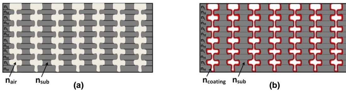
Fig. 1 Schematic cross-section of the 1D PC (rugate filter) with high and low refractive layers without (a) and with ALD coating (b)
