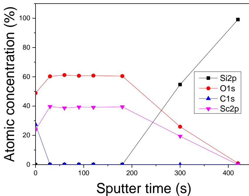
XPS depth profile of a \text{Sc}_2\text{O}_3 film grown at 275 °C from Sc-07 and water.
