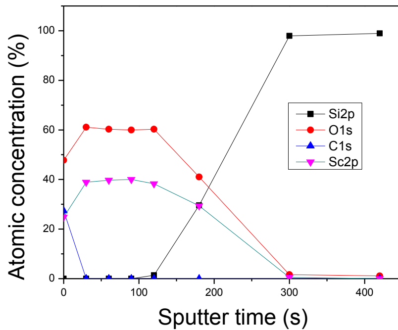
XPS depth profile of a \text{Sc}_2\text{O}_3 film grown at 230 °C from Sc-07 and water.
