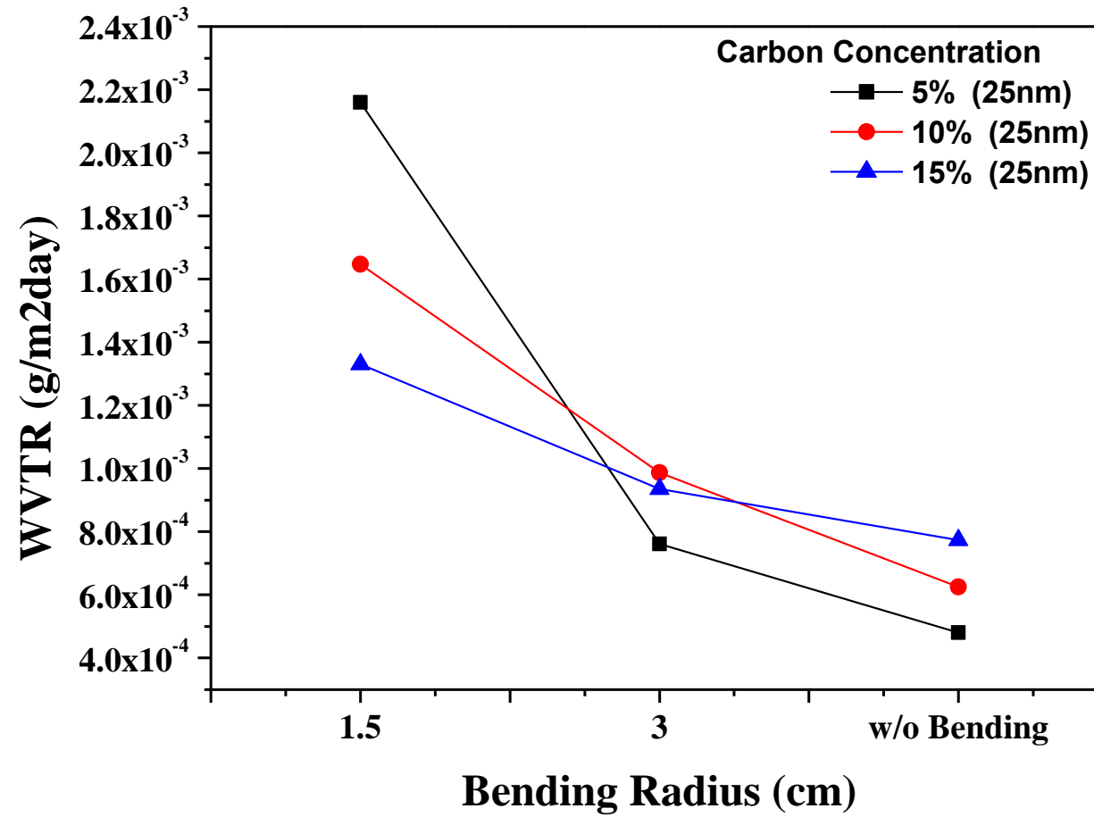
Figure. 1 WVTR vs. bending radius of Al 2 O 3 films by electrical Ca Test at 85°C and RH 85%
