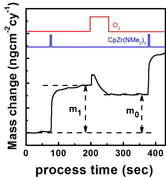
Figure 1. Frequency change with process time by alternating injections of CpZr(NMe 2 ) 3 and O 3 .
