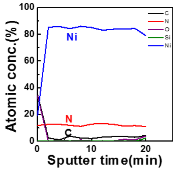
Figure 1. XPS depth profile of the PEALD nickel film deposited at 150°C.
