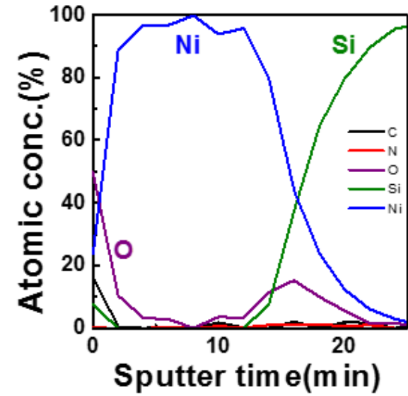
Figure 2. XPS depth profile of the PEALD nickel film after annealing in H 2 at 400°C.
