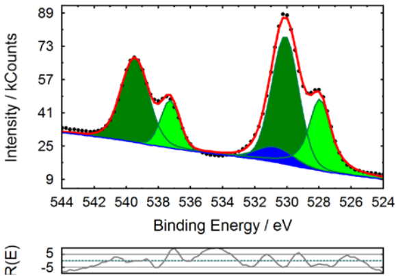
Fig. 1: XPS spectrum of the Sb 3d region of an Sb ALD film contaminated in air (dark green: Sb (oxidized), green: Sb (metallic), blue: oxygen)
