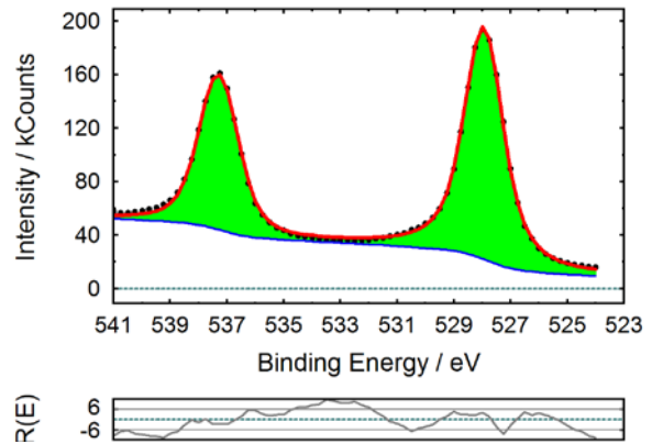
Fig. 2: XPS spectrum of the Sb 3d region of an Sb ALD film after 12s Ar sputtering (green: Sb (metallic))
