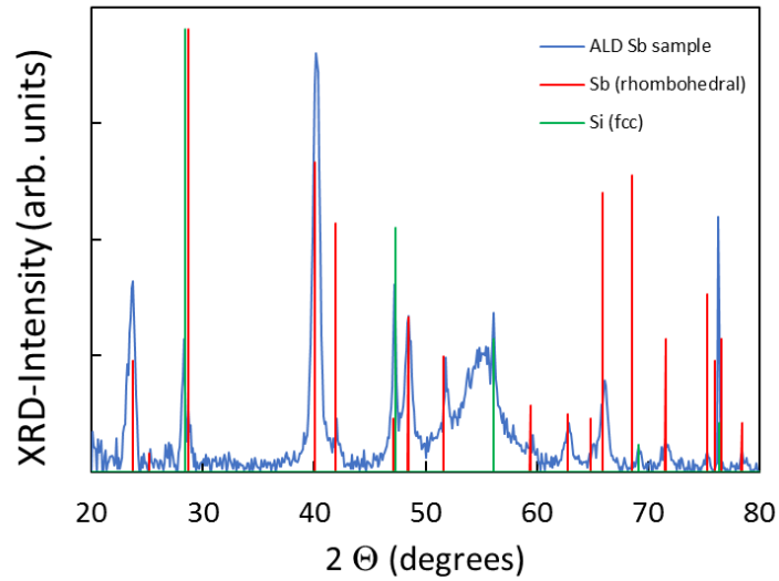
Fig. 3: Diffraction pattern of pure ALD Sb film deposited on silicon substrate without further annealing.
