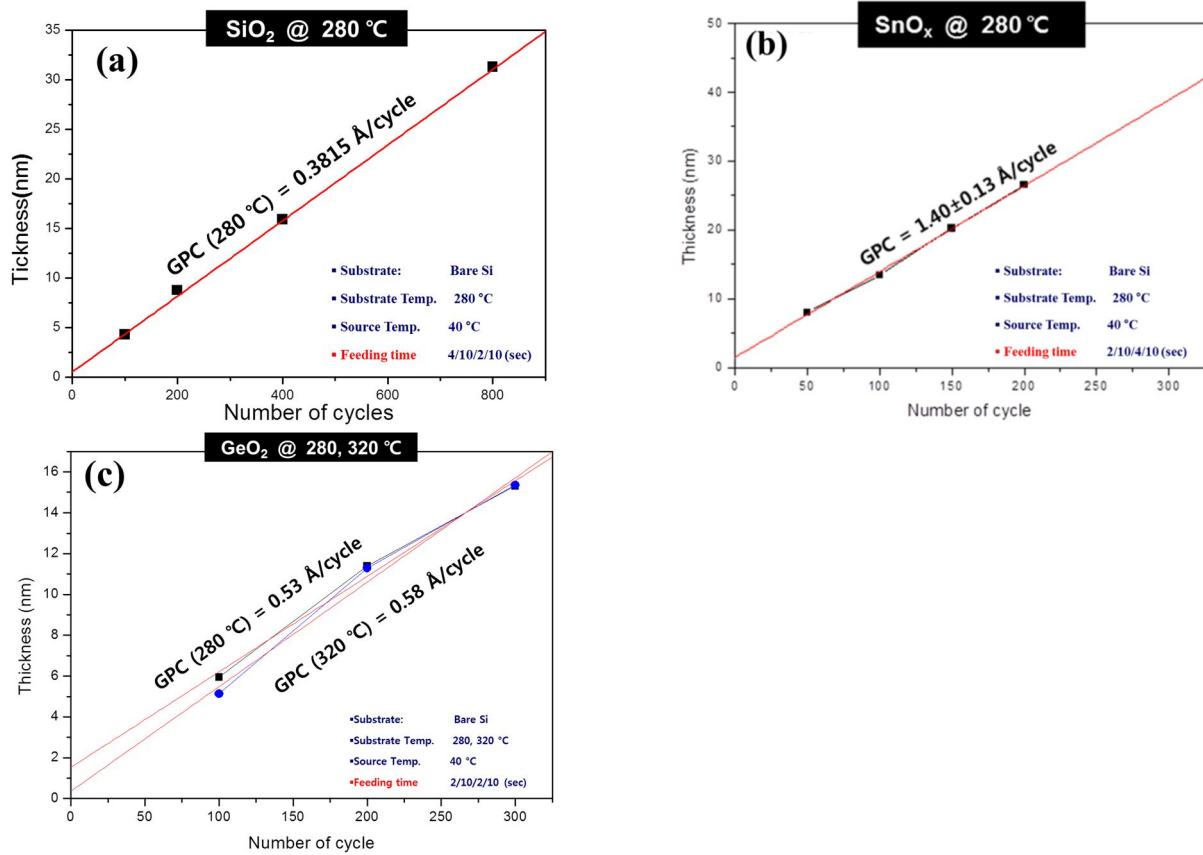
Figure 1. (a) Deposition rates of SiO x , (b) deposition rates of SnO x and (c) deposition rate of GeO x film deposited by O 3 .
