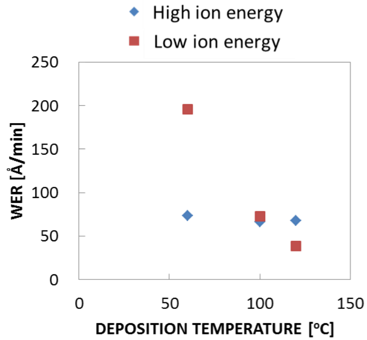
Fig. S1 Temperature dependence of WER of TiO 2 films
