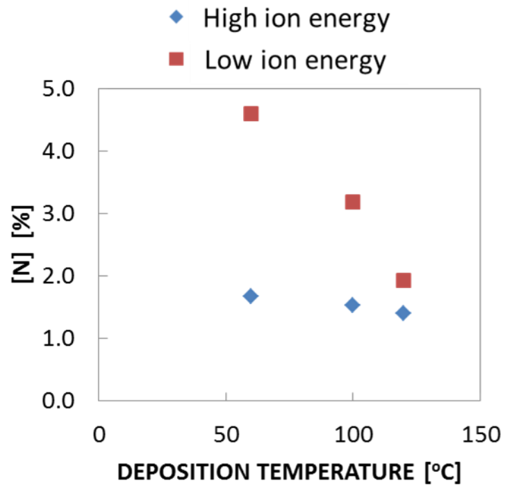
Fig. S2 Temperature dependence of nitrogen composition of TiO 2 films
