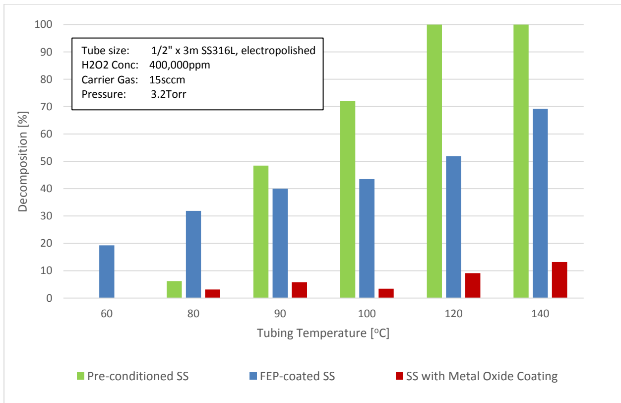
Figure 1. Decomposition of Anhydrous Hydrogen Peroxide on various materials.
