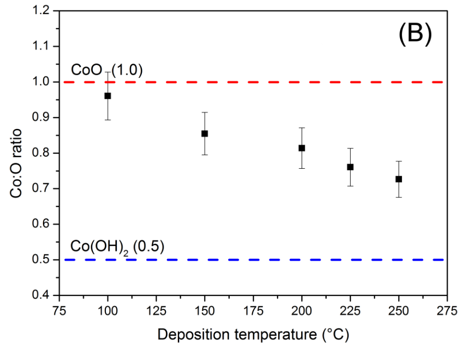
Figure 1. The effect of deposition temperature on GPC (A) and Co:O ratio in the films (B).
