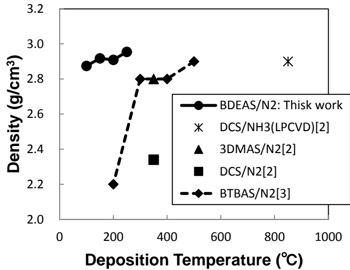
Fig. 1 SiN film density as a function of deposition temperature.
