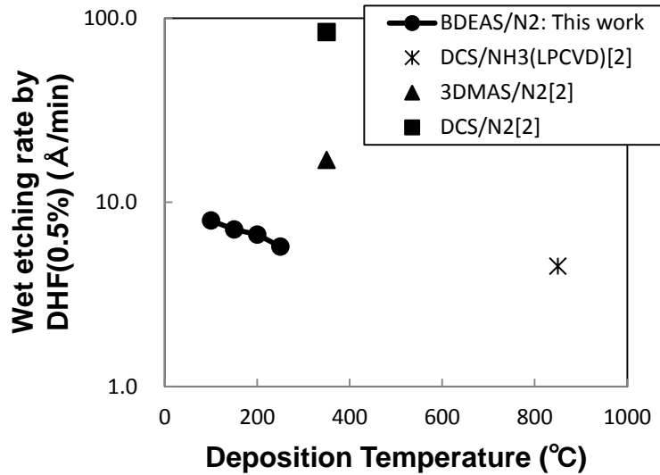
Fig. 2 WER as a function of deposition temperature.
