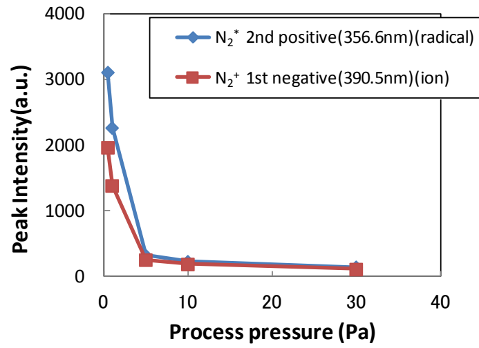
Fig.1 Emission intensities of N 2 radical and ion as a function of process pressure.
