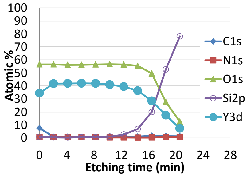
Figure 1: XPS depth profile of Y_2O_3 film
