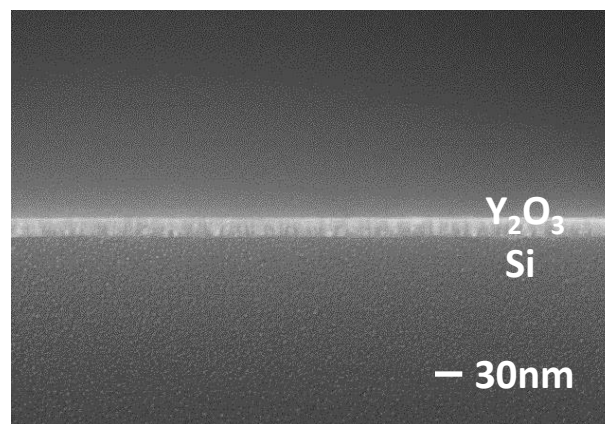
Figure 2: XSEM image of Y_2O_3 film
